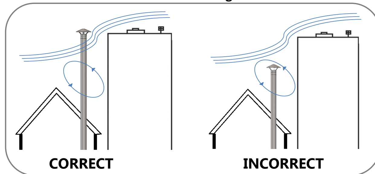
2nd Case.- Chimney cowl above the ridge, but with nearby high building.
